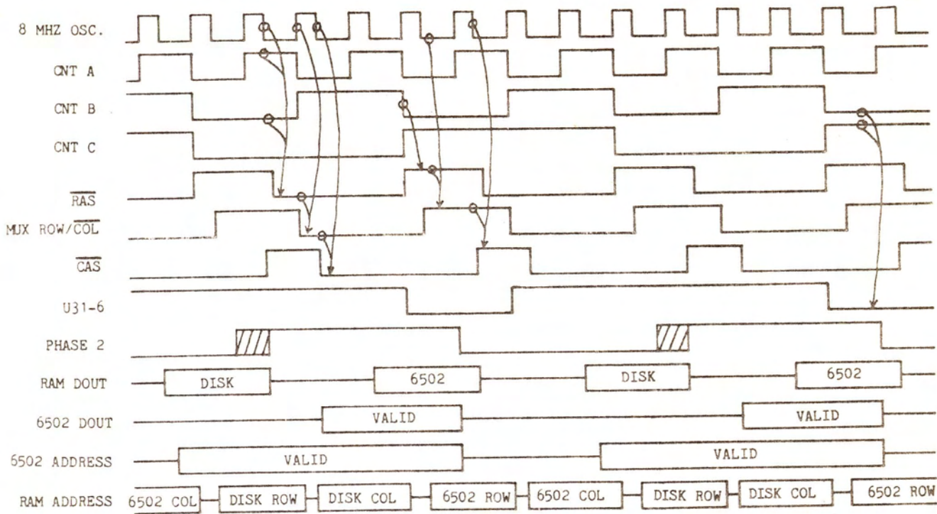
MEMORY CYCLE TIMING DIAGRAM
