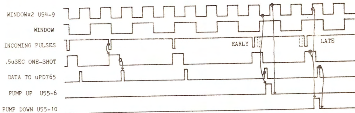
DATA SEPARATOR TIMING DIAGRAM
